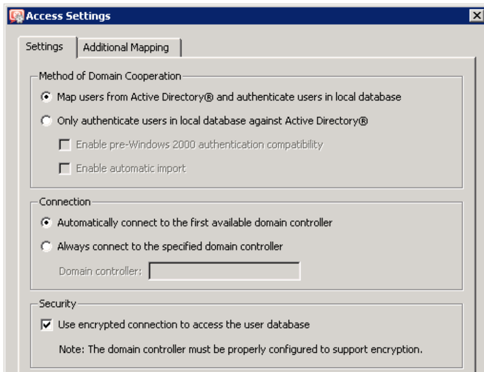
Figure 15.13 Advanced options for cooperation with the Active Directory.
