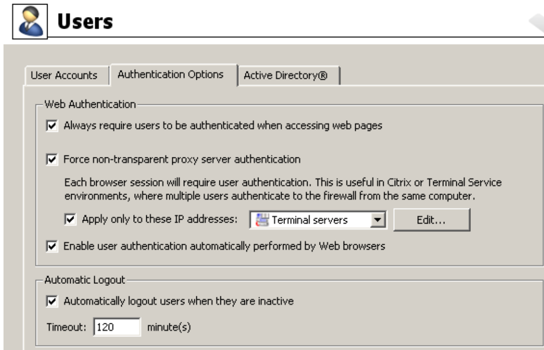
Figure 10.1 User Authentication Options
