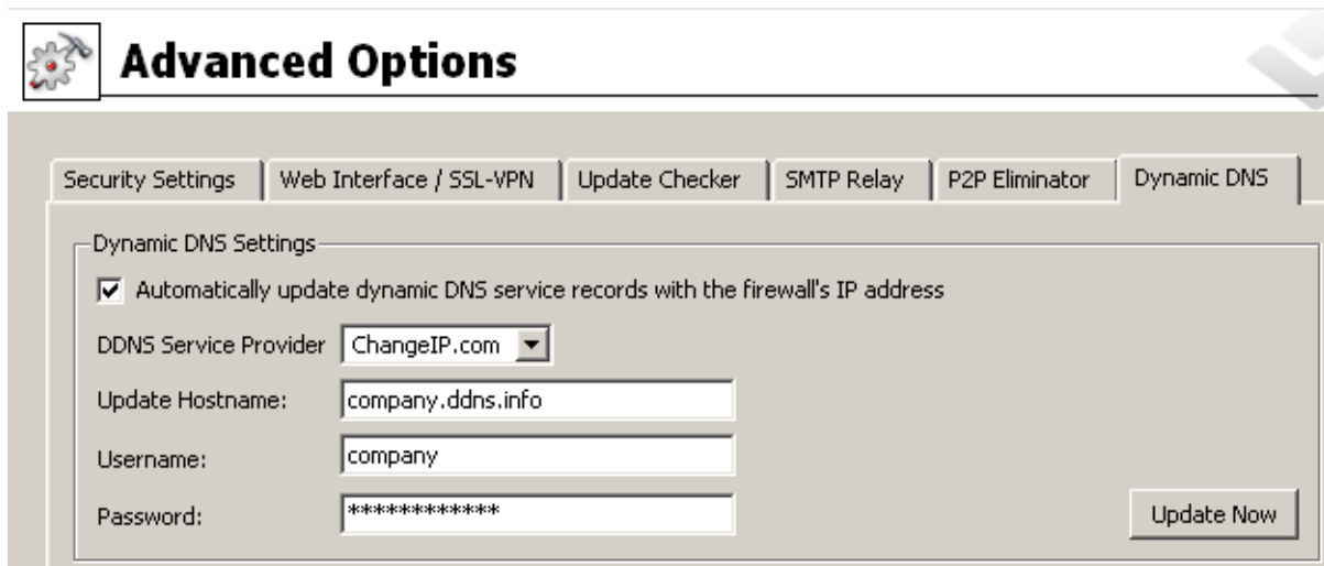
Figure 8.14 Setting cooperation with dynamic DNS server
