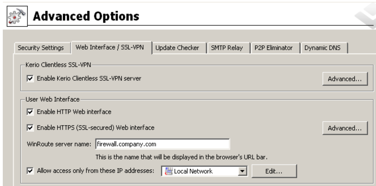
Figure 25.2 Configuration of WinRoute's Web Interface
