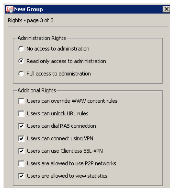
Figure 15.19 Creating a user group — members' user rights
