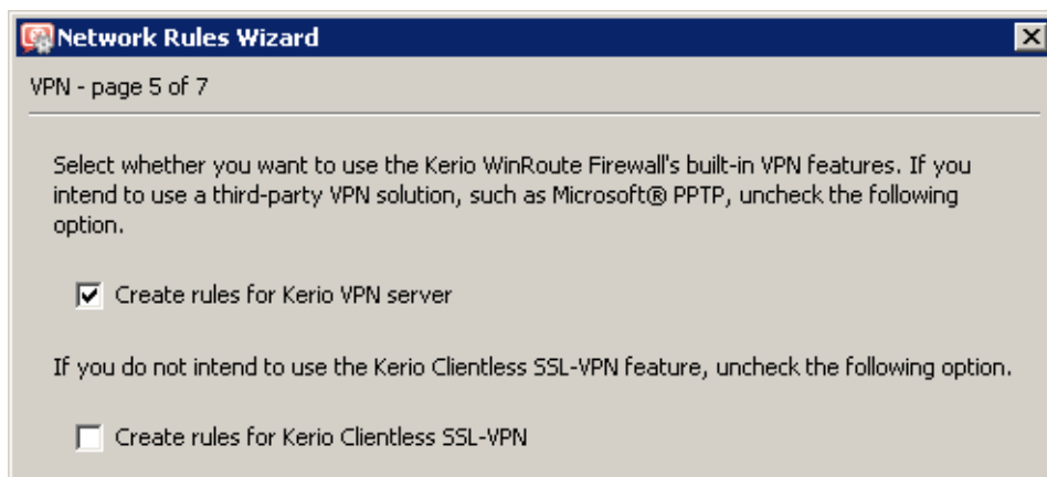
Figure 23.43 The London filial office — creating default traffic rules for Kerio VPN
