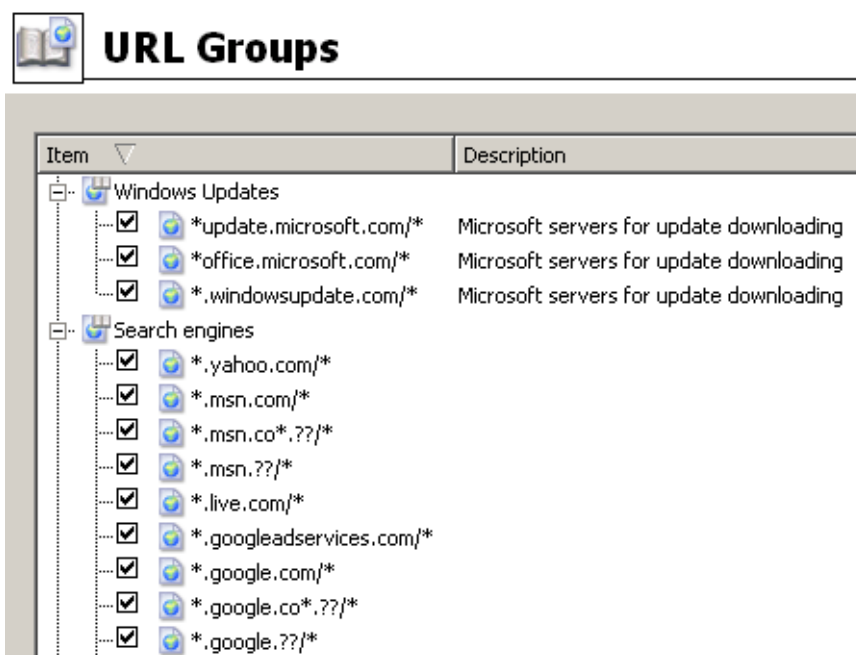
Figure 14.9 URL Groups
