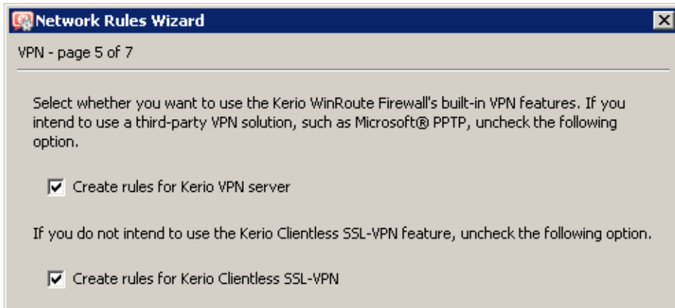
Figure 23.15 Headquarter — creating default traffic rules for Kerio VPN
