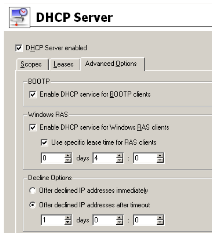
Figure 8.13 DHCP server — advanced options
