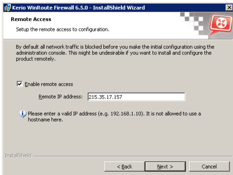
Figure 2.4 Initial configuration — Allowing remote administration
